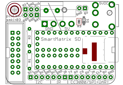
SmartMatrix SD Shield Rev V1
